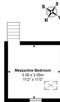
Annexe Mezzanine Floor Approximate Floor Area - 11.4 m 2 ... 122 ft 2
